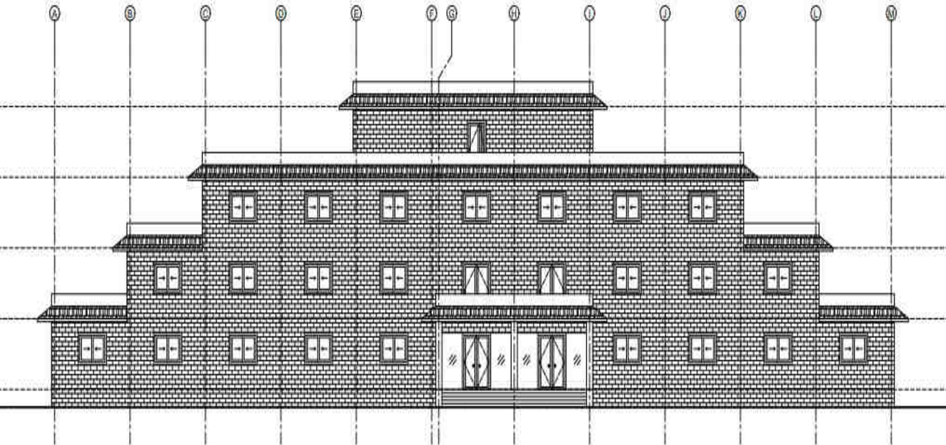
Front Elevation
