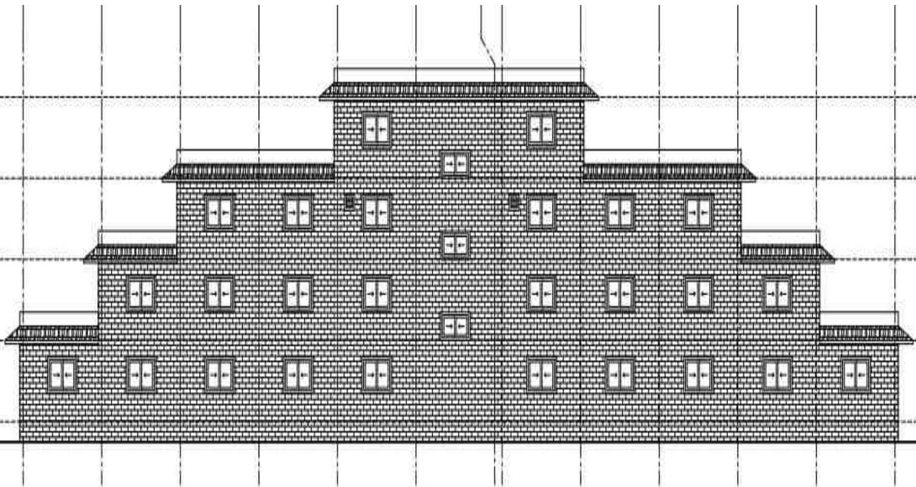
Back Elevation
